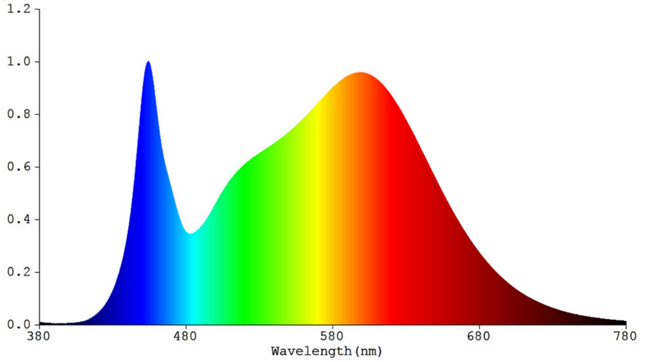
Spectrum
