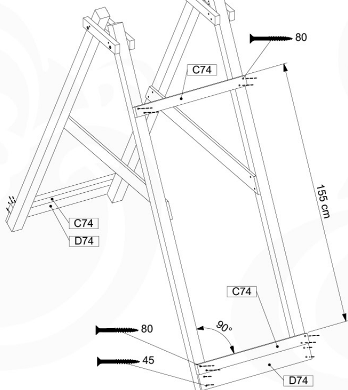
Climb Frame 200
