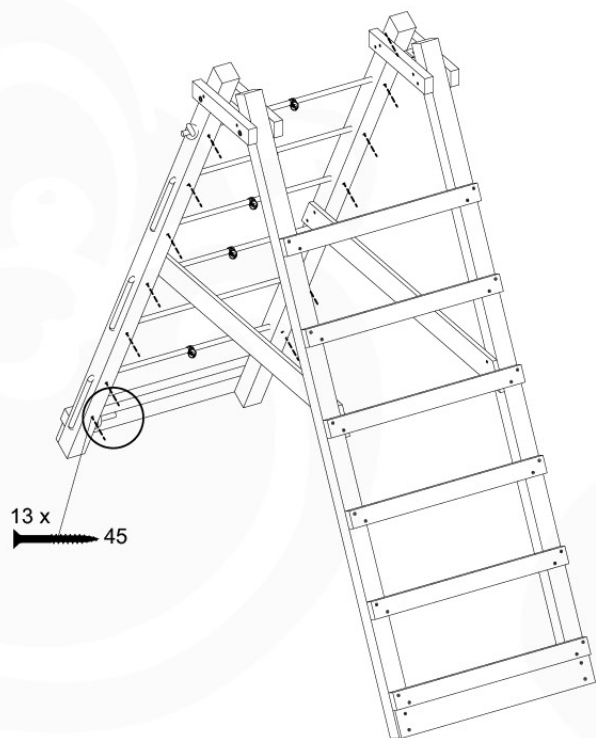
Climb Frame 200
