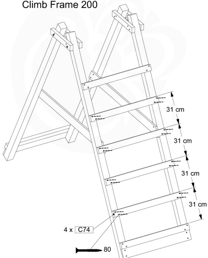
Climb Frame 200
